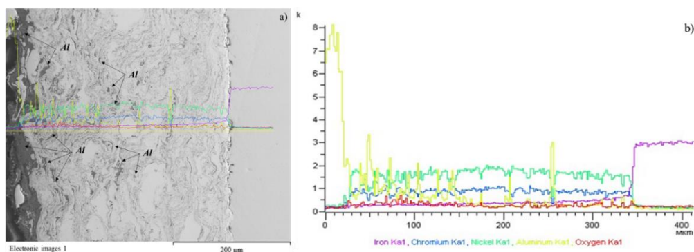
Figure 2 – SEM cross-section images (a) and element distribution (b) as a function of depth in the Ni–Cr–Al gradient coating.
