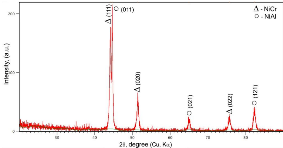
Figure 1 – Diffractograms of Ni–Cr–Al gradient coatings obtained by detonation spraying
