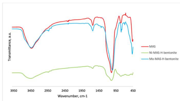
Figure 6 – FT-IR spectra of mesoporous aluminosilicate (MAS) and bifunctional catalysts based on it. Error bars depict 95% confidence intervals
